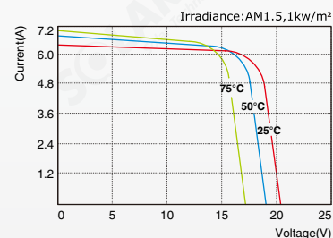
SIM100-12 I-V Curves
